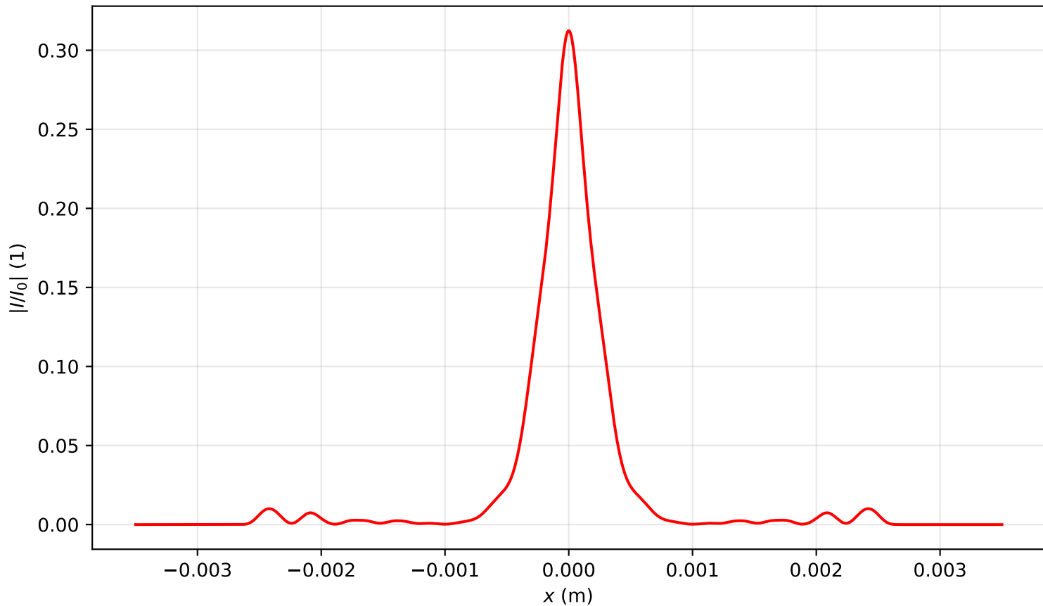
Intensity profile I(x, y = 0, z = 2.229)/I_0 , P_{in}=6.0P_{cr} , artificial time
